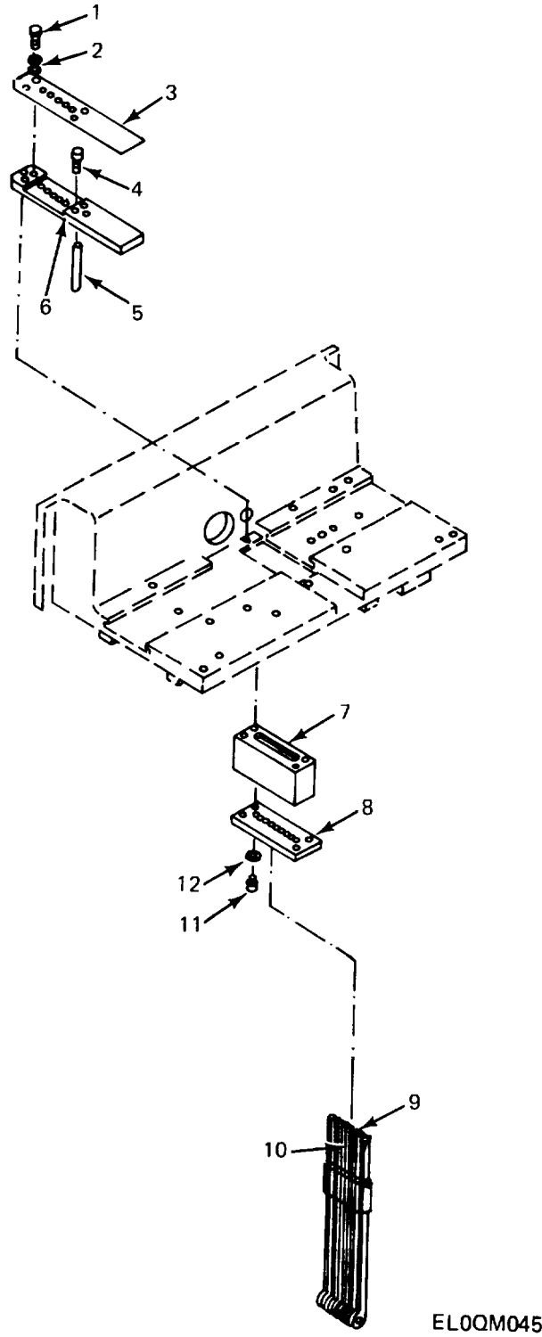
Figure 38. Head, Punch Assembly.
