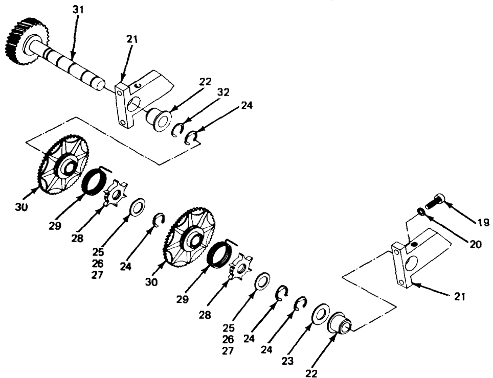
CLUTCH AND SLEEVE ASSY.
