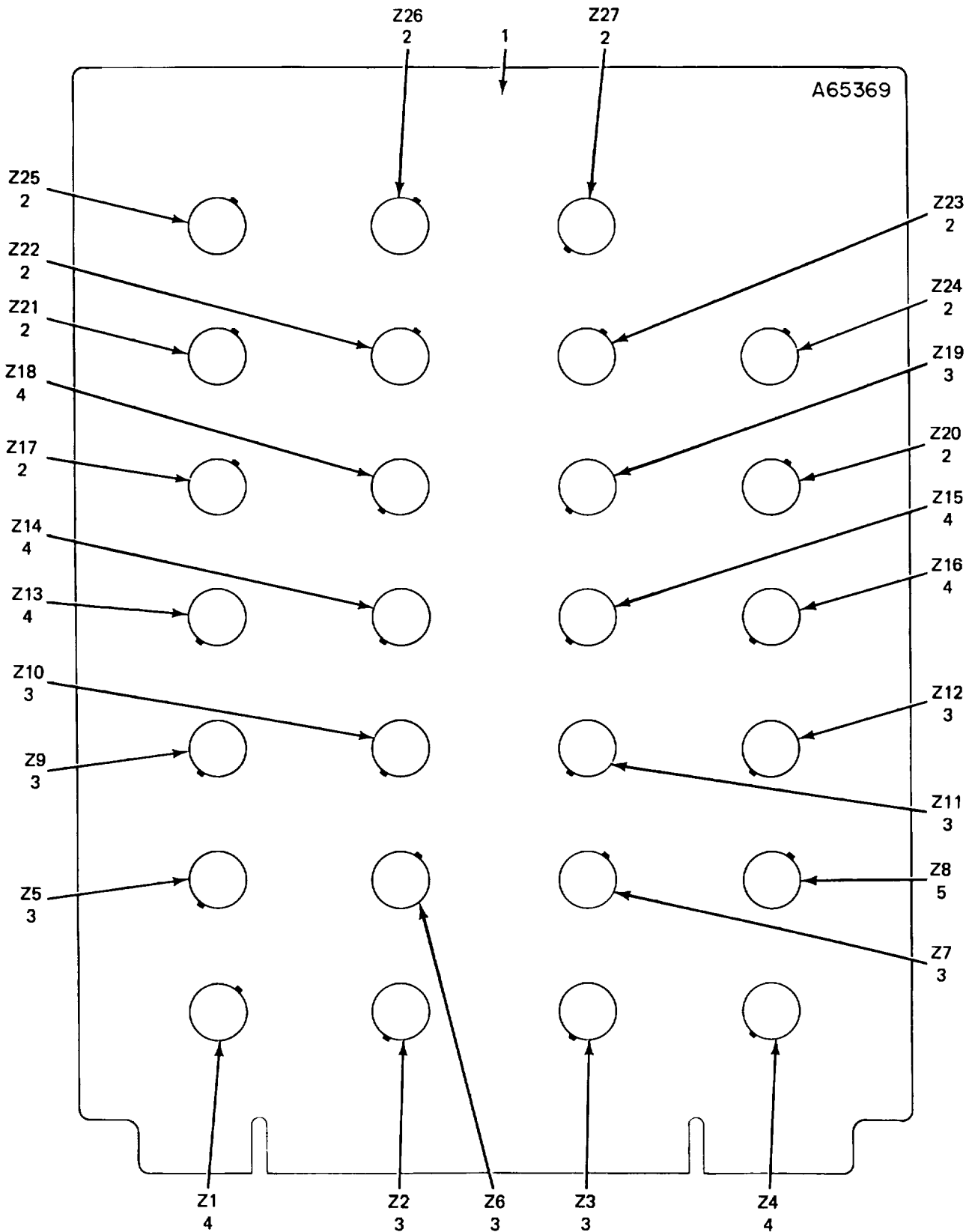
Figure 11. Circuit Card Assembly A1A7.
