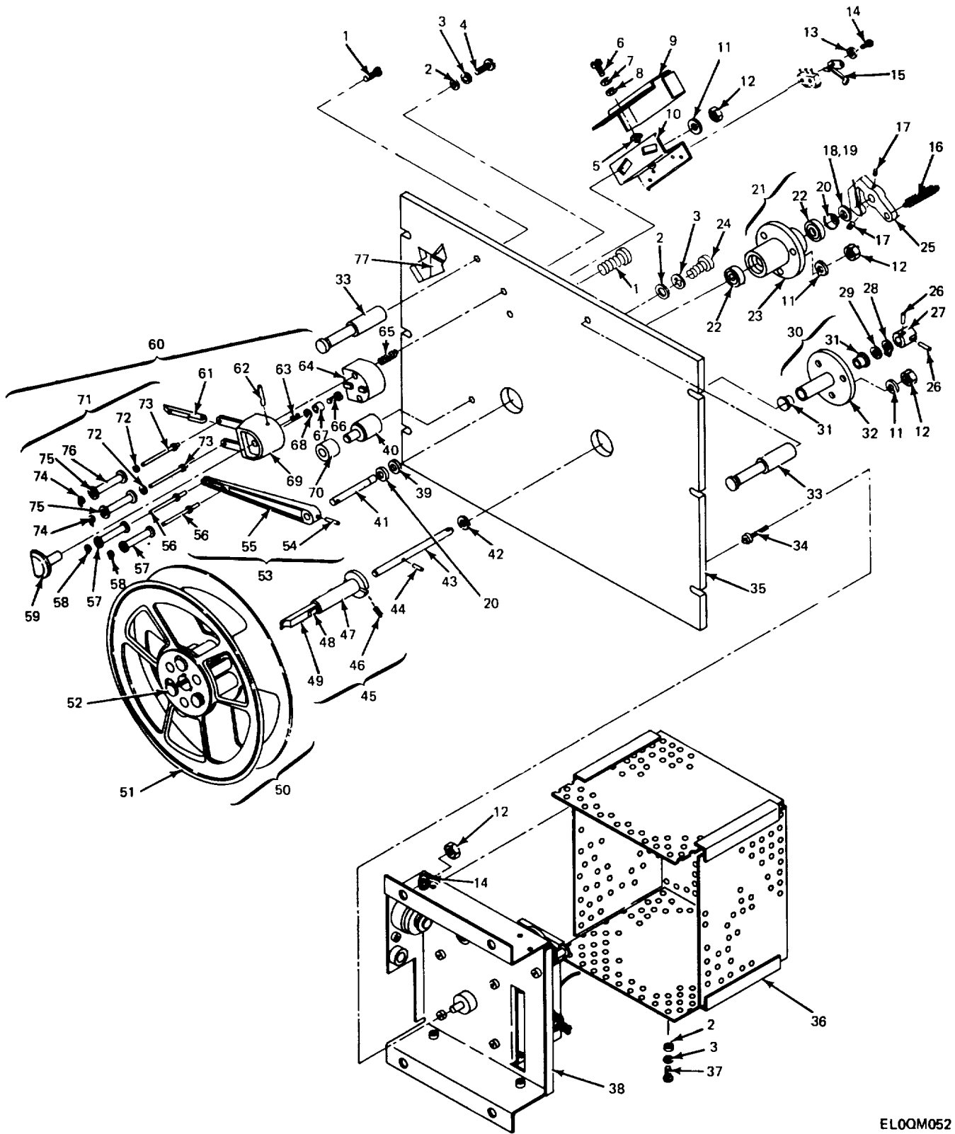
Figure 45. Tape Reeler B2.
