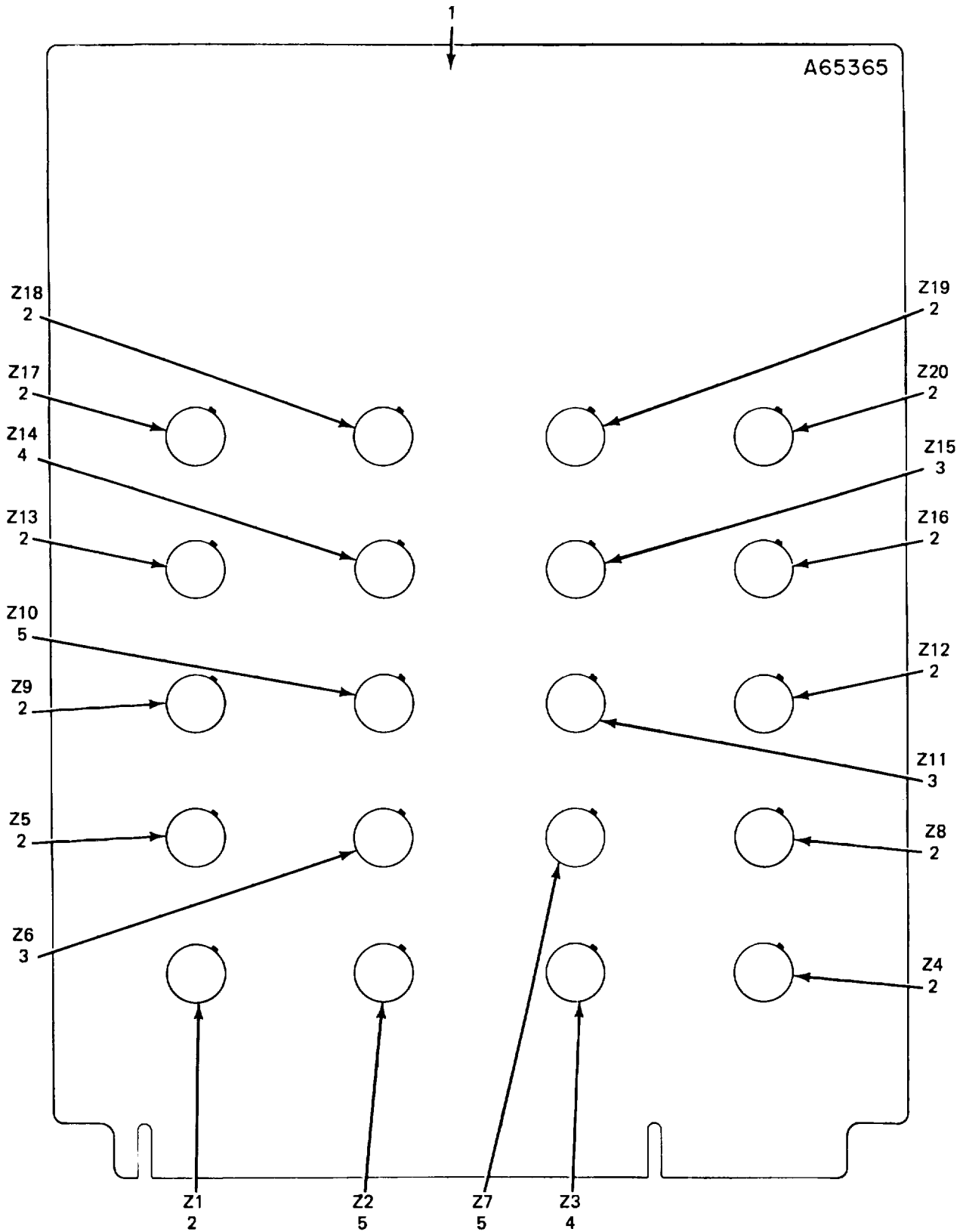
Figure 10. Circuit Card Assembly A1A6.
