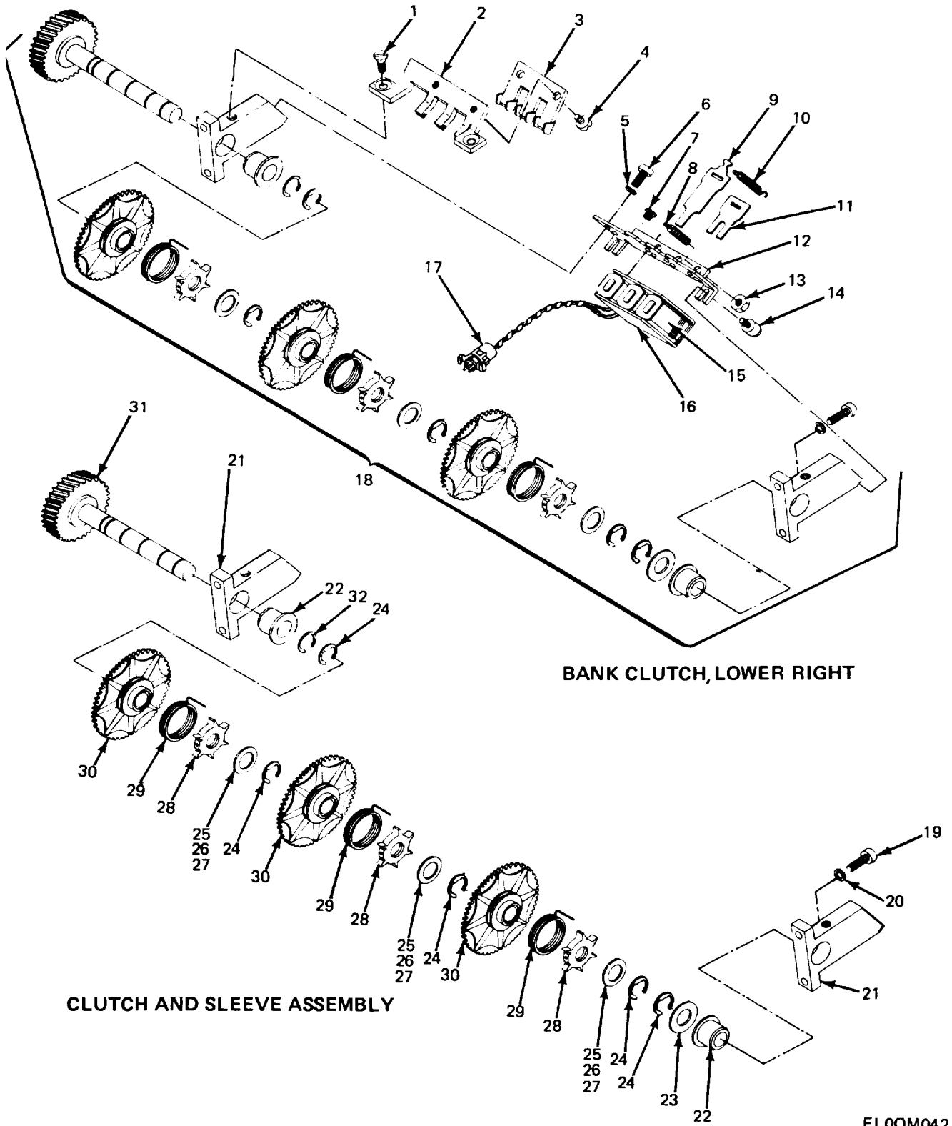
Figure 35. Bank Clutch, Lower Right and Clutch and Sleeve Assembly.
