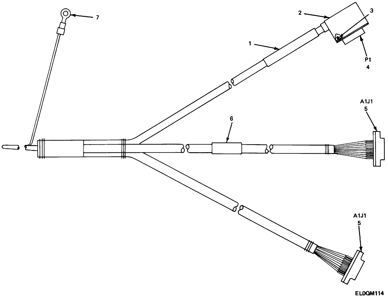
Figure 95. Cable Assembly (40638G1).
