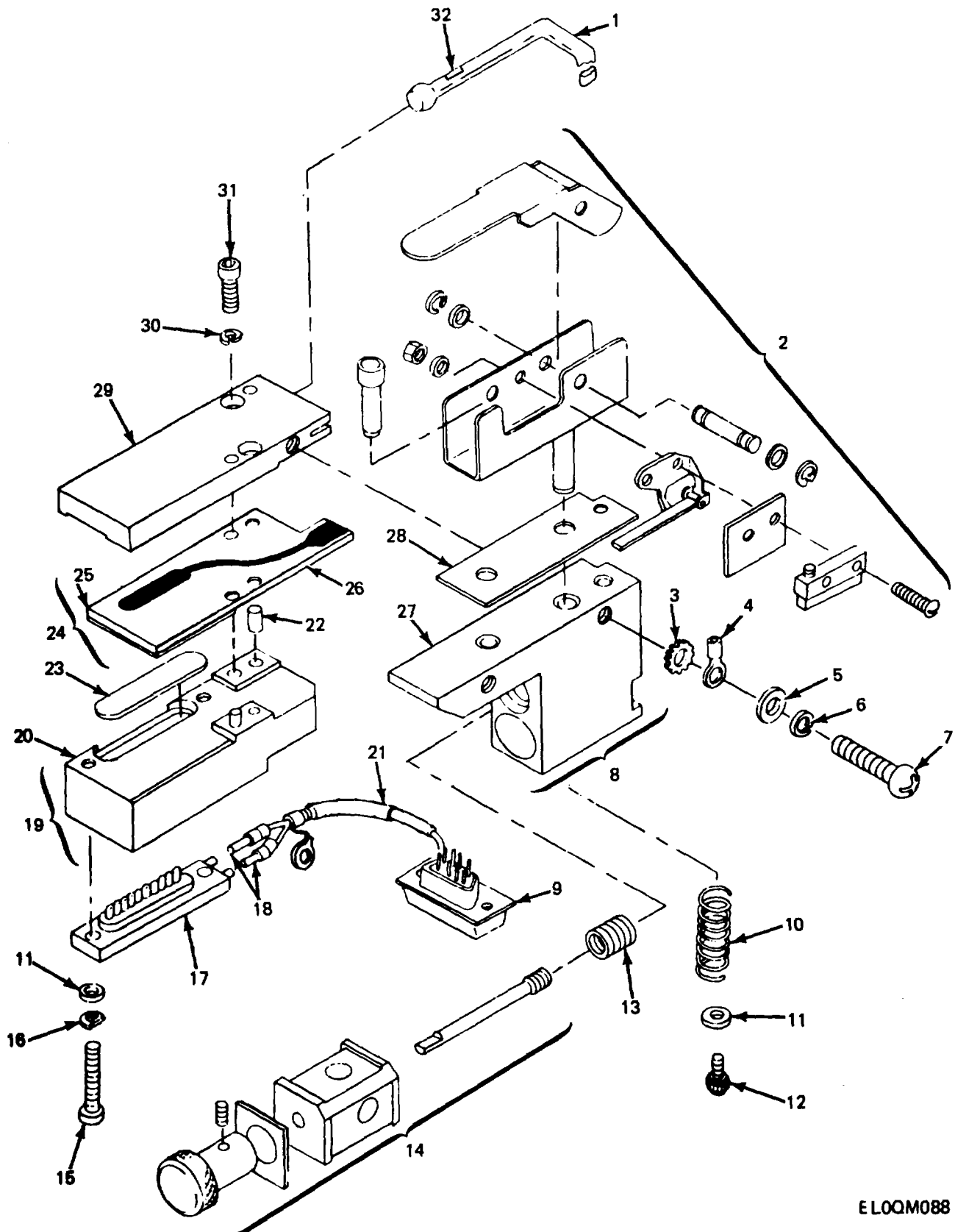
Figure 76. Tape Reader Assembly
