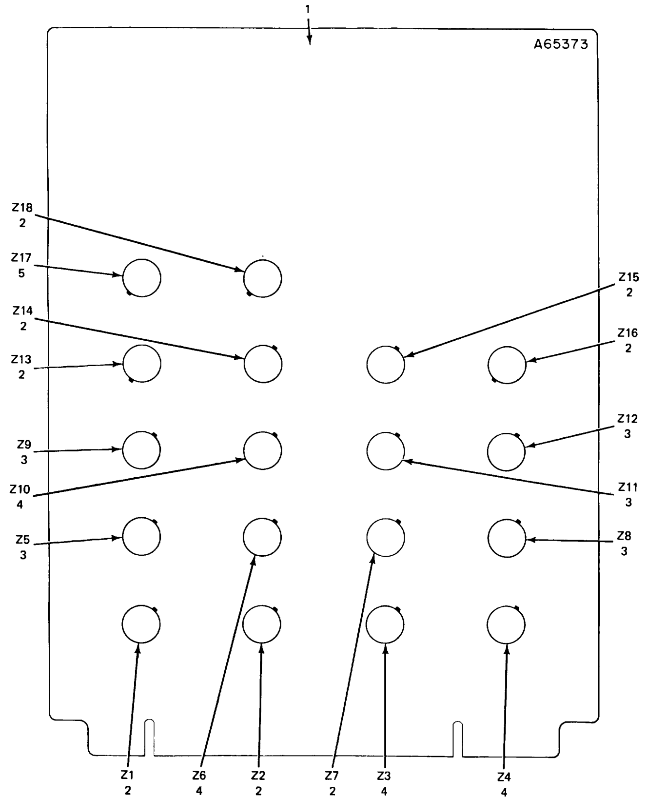
Figure 12. Circuit Card Assembly A1A19.
