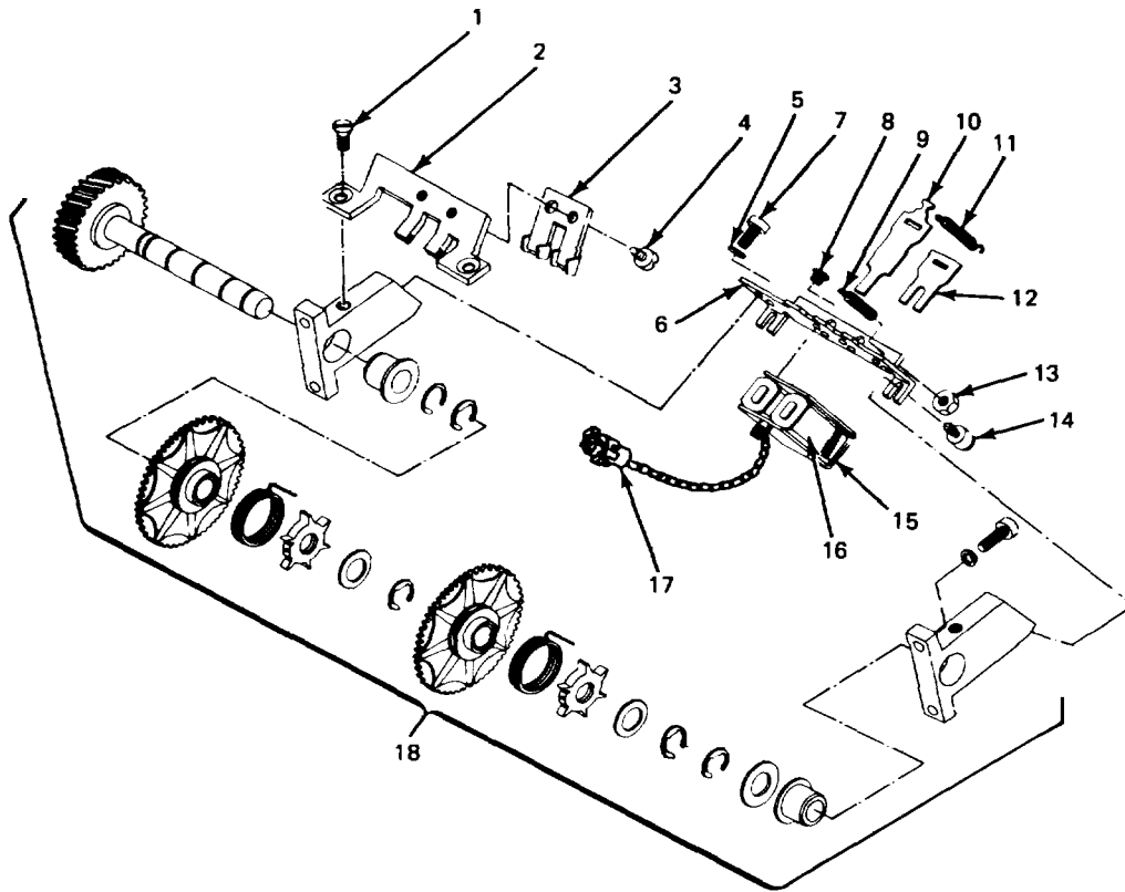
LOWER LEFT BANK CLUTCH
