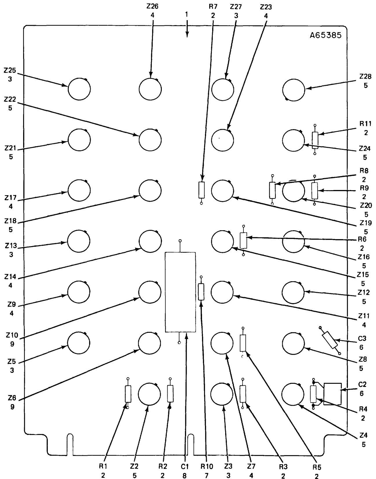
Figure 14. Circuit Card Assembly A1A10.
