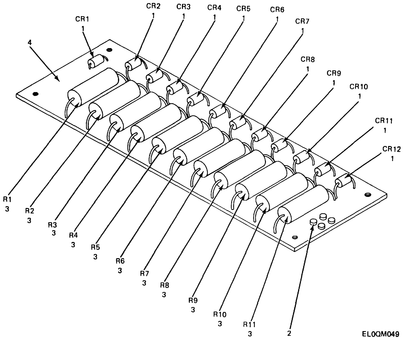
Figure 42. Circuit Card Assembly (833070).
