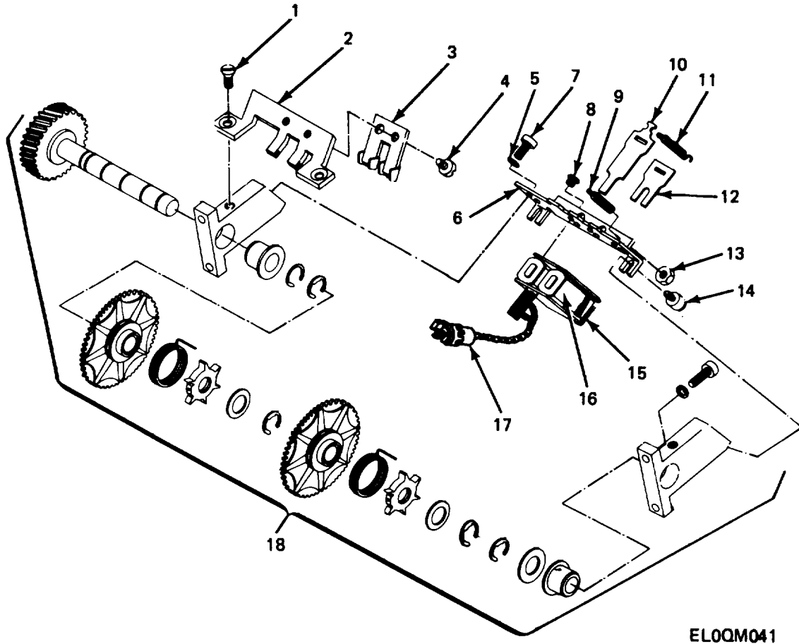
Figure 34. Bank Clutch, Upper Left.
