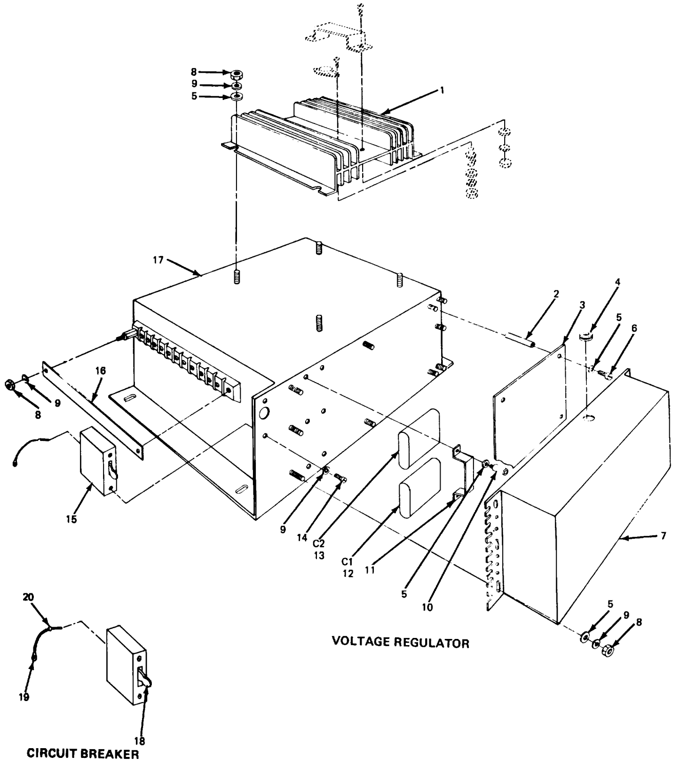
Figure 61. Voltage Regulator Assembly VR1 and Circuit Breaker Assembly.
