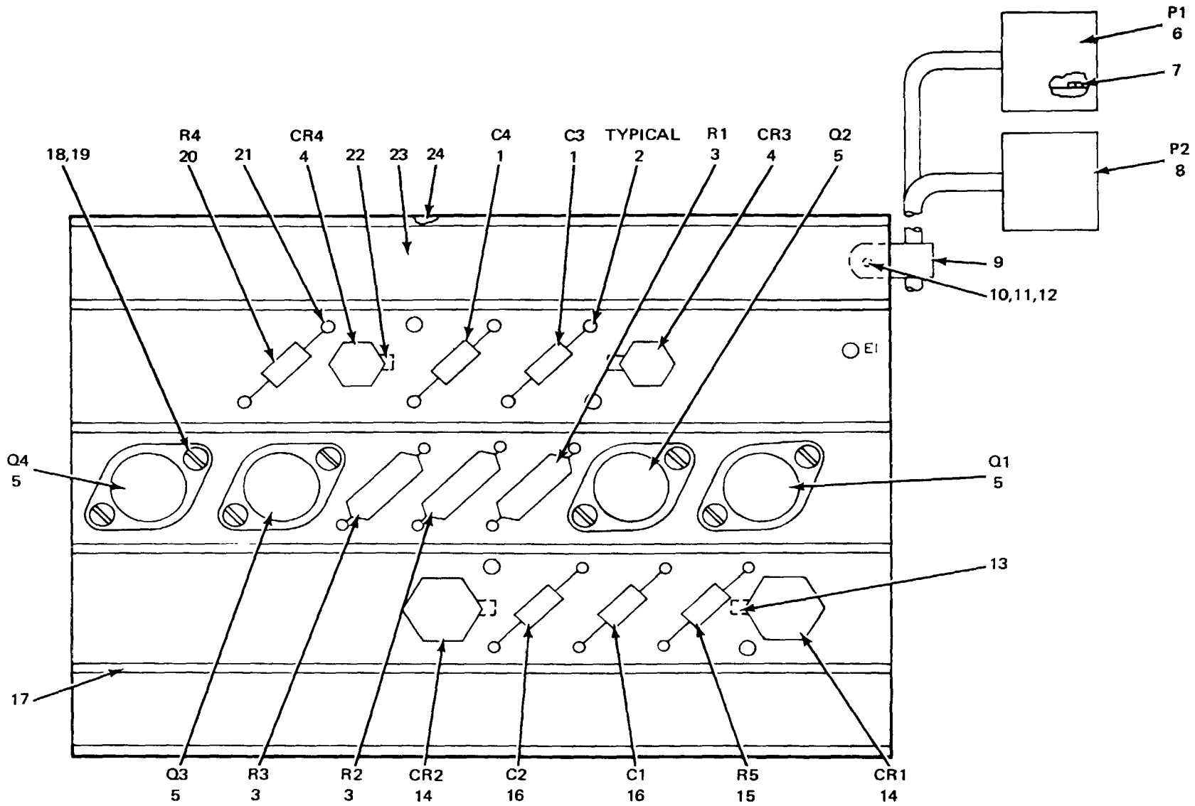
Figure 52. Heat Sink Subassembly PS1A4.
