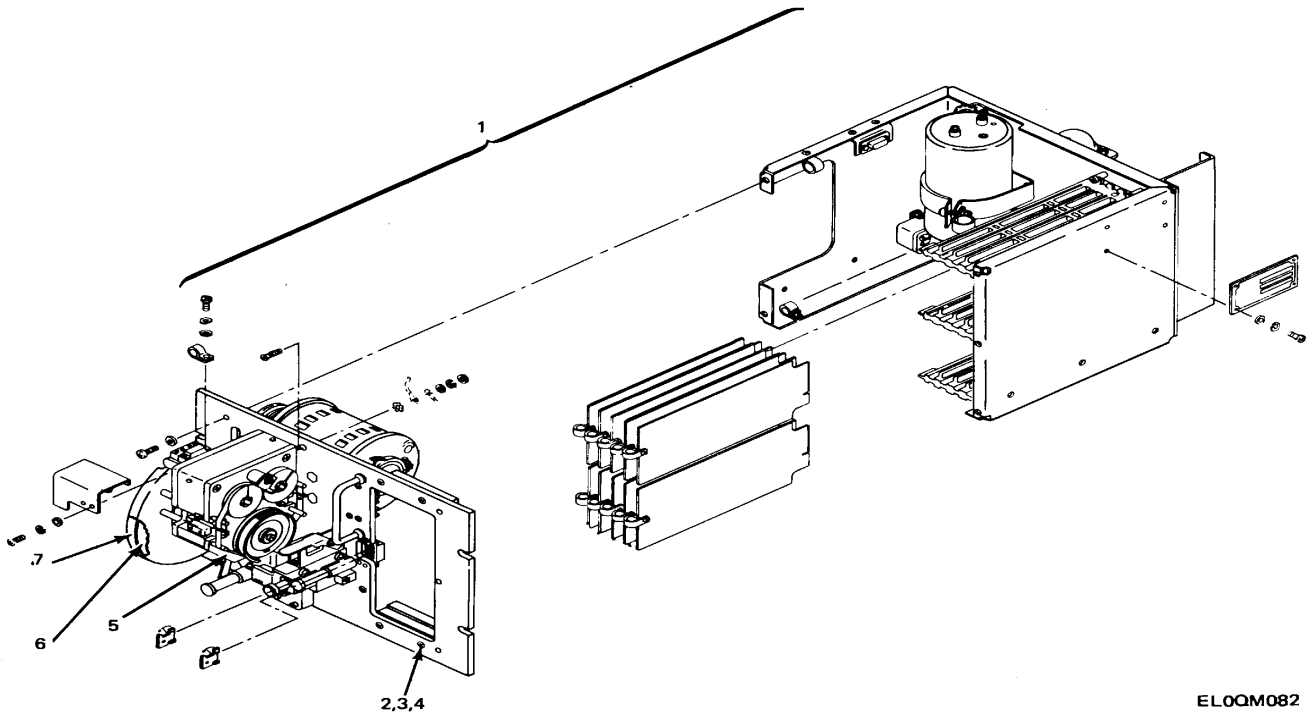
Figure 71. Printer Interpreter Assembly A3.
