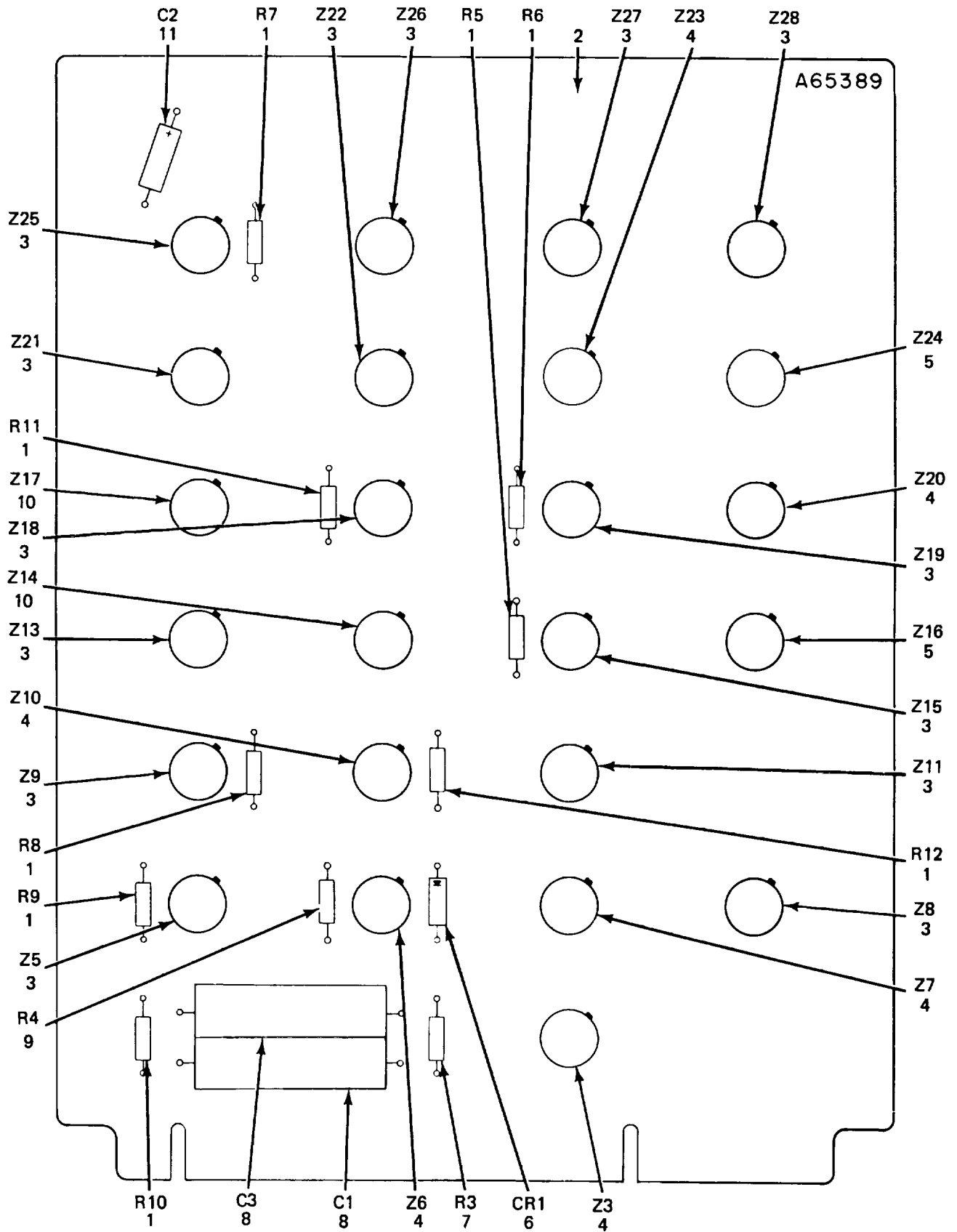
Figure 15. Circuit Card Assembly A1A11.
