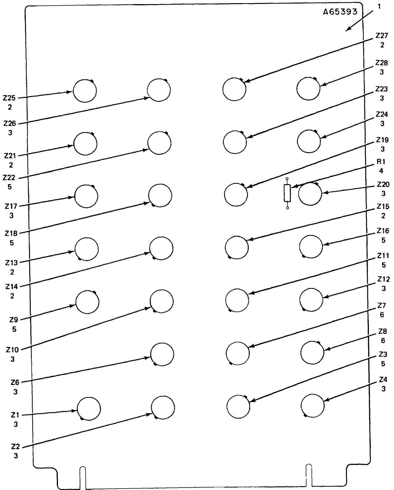
Figure 16. Circuit Card Assembly A1A4.
