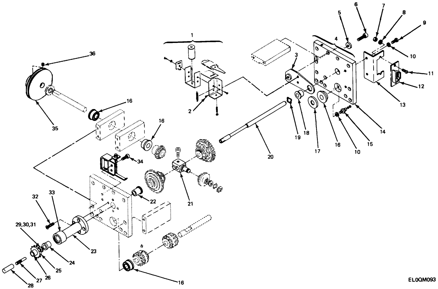
Figure 81. Tape Drive Assembly.
