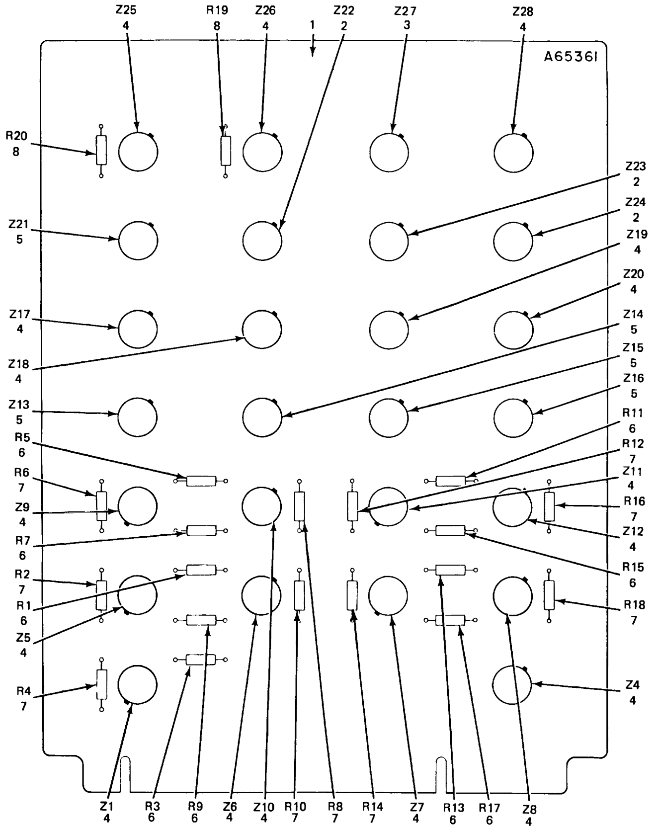
Figure 9. Circuit Card Assembly A1A5.
