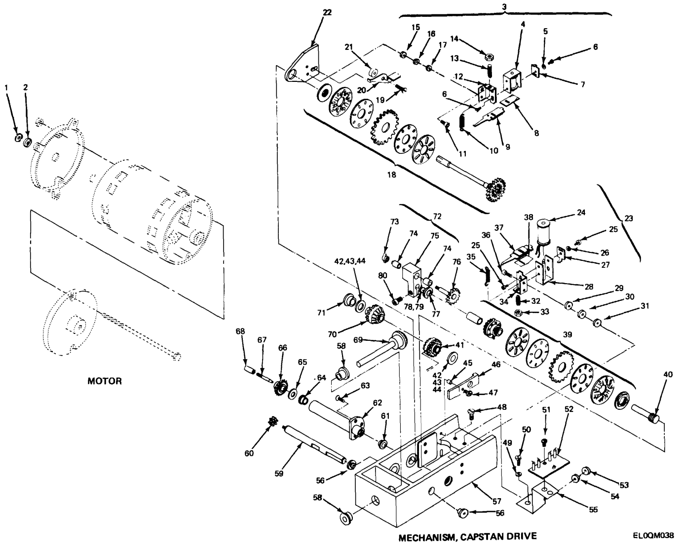
Figure 31. Motor and Mechanism, Capstan Drive.
