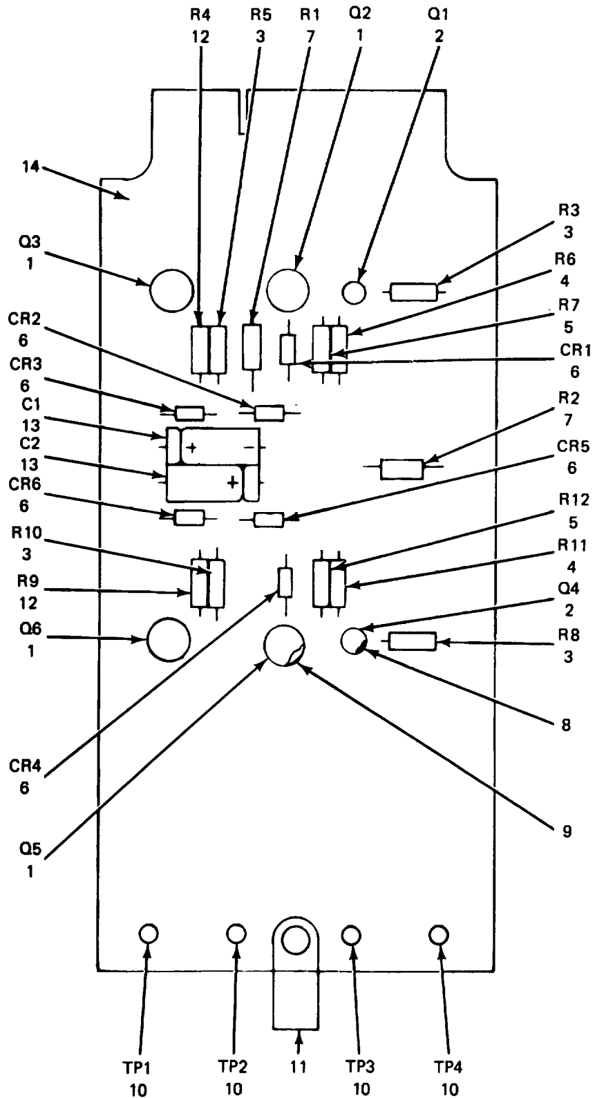
Figure 84. Circuit Card Assembly A3A2A0.
