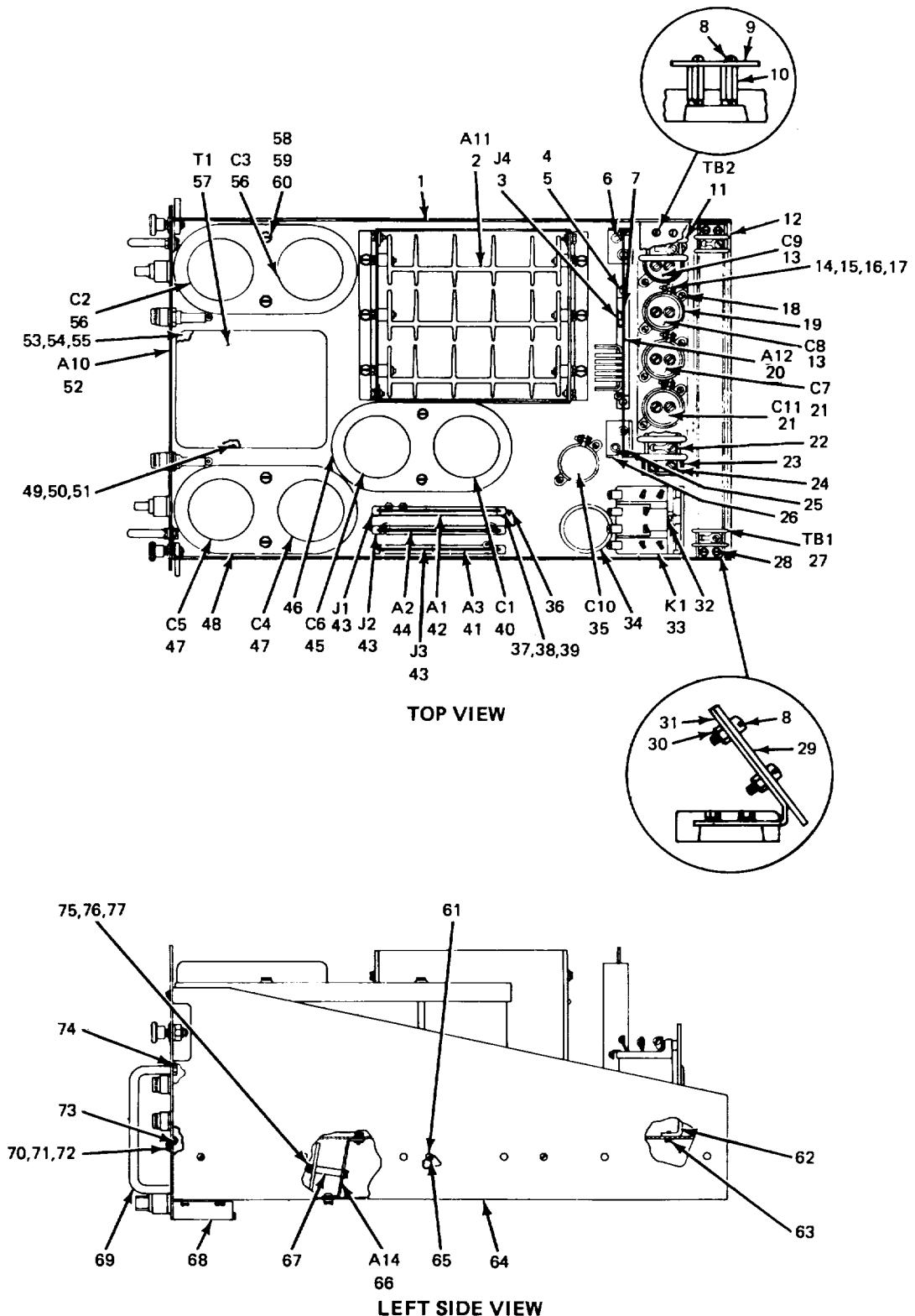
Figure 47. Power Supply PS1.
