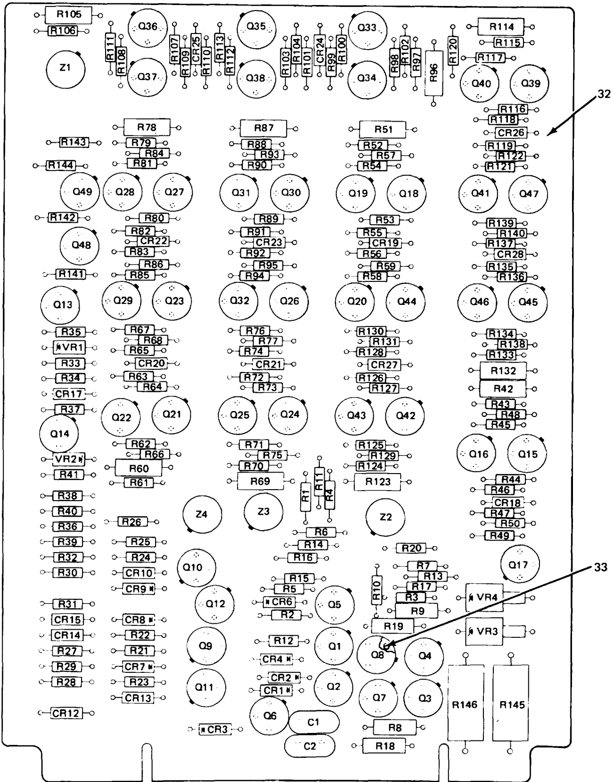
CIRCUIT CARD NO. 65201-001
