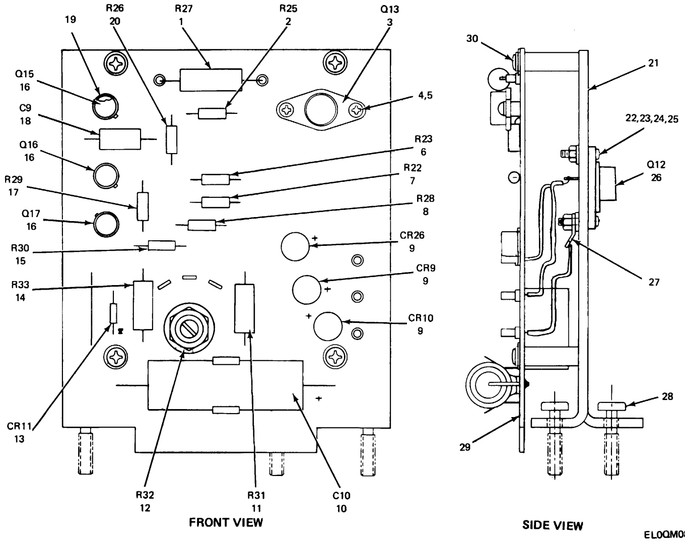
Figure 69. Circuit Card Assembly (12-890140-002).
