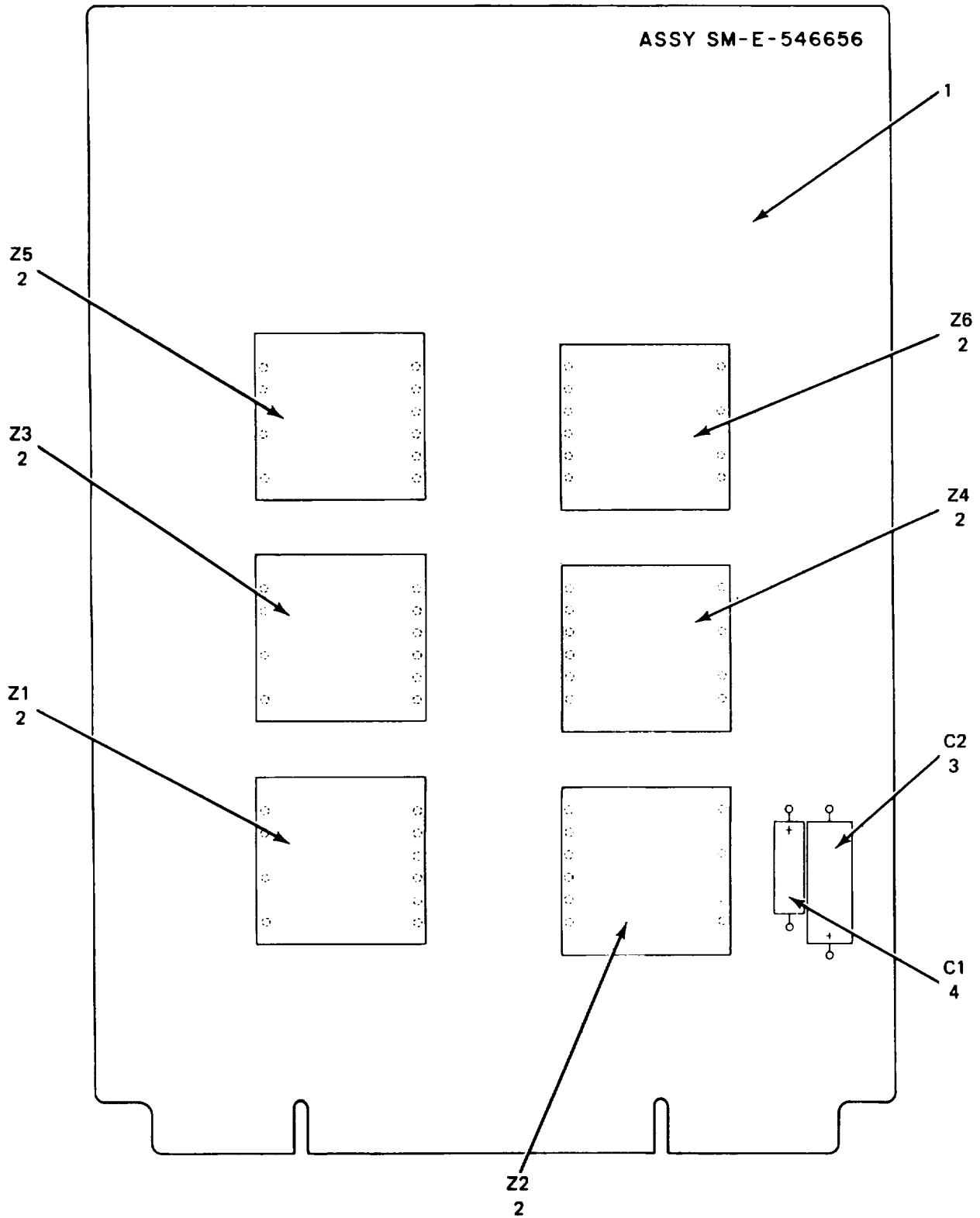
Figure 18. Circuit Card Assembly A1A20.
