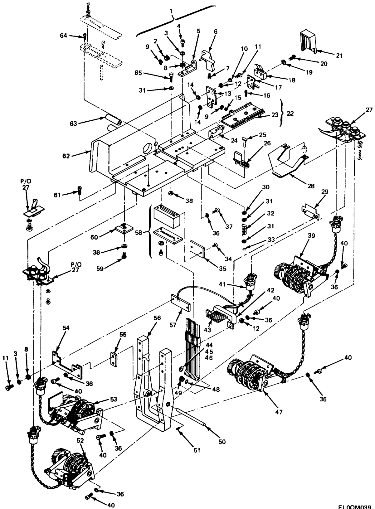
Figure 32. Mechanism, Punch
