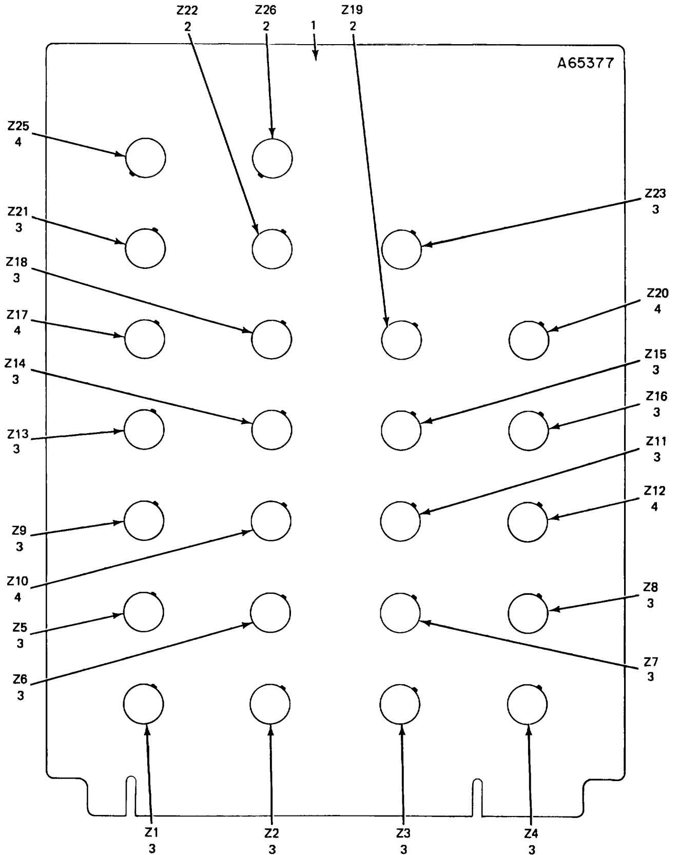
Figure 13. Circuit Card Assembly A1A9.
