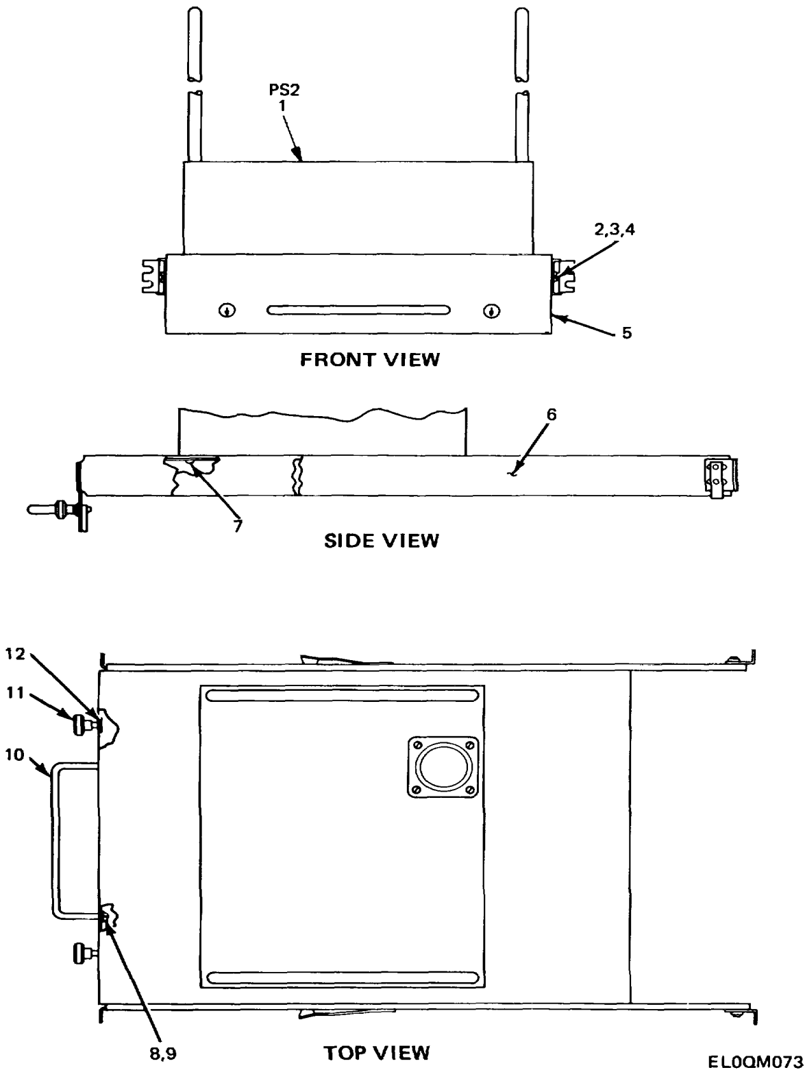
Figure 64. Power Supply Assembly PS2.
