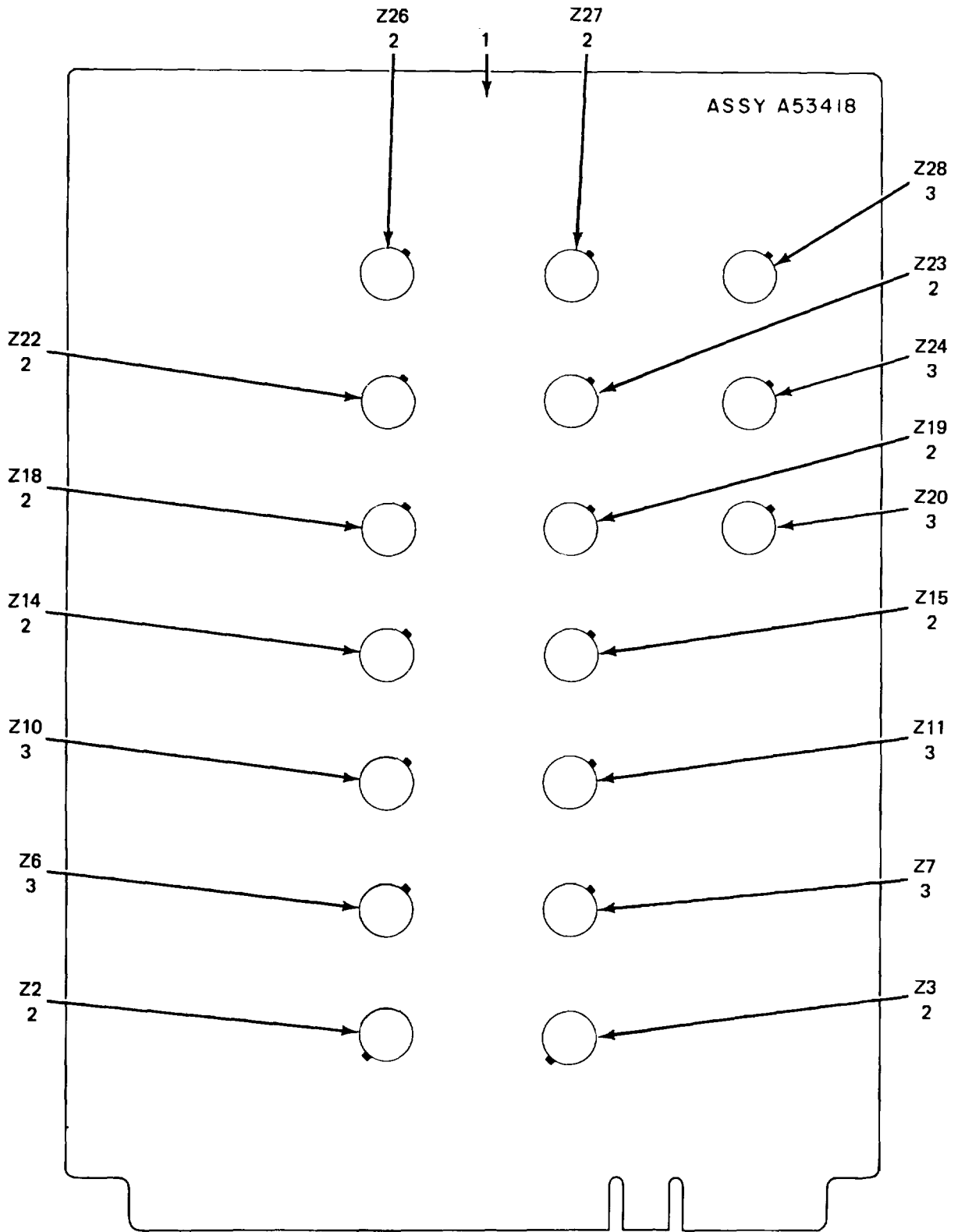
Figure 3. Circuit Card Assembly A1A14.
