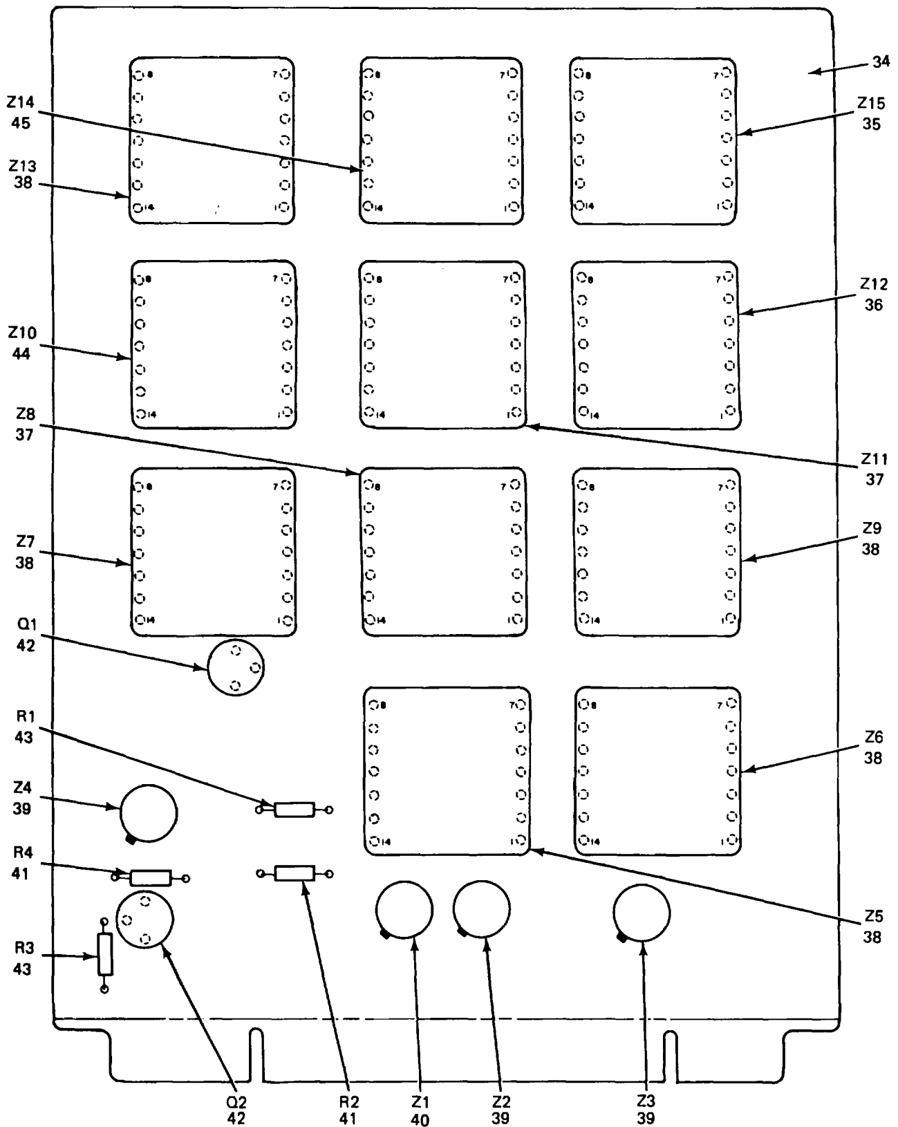
Figure 8. Circuit Card Assembly A1A1 (Sheet 4 of 4).
