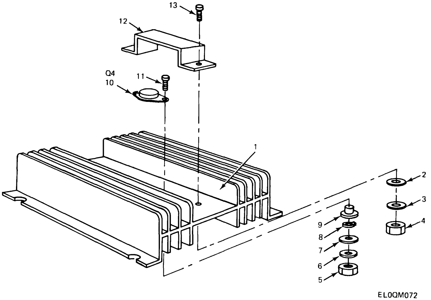
Figure 63. Heat Sink Assembly (W-7712-26).
