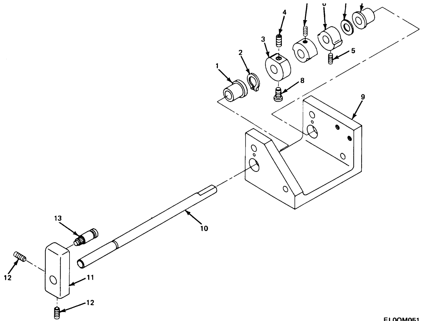
Figure 44. Sensing Assembly.
