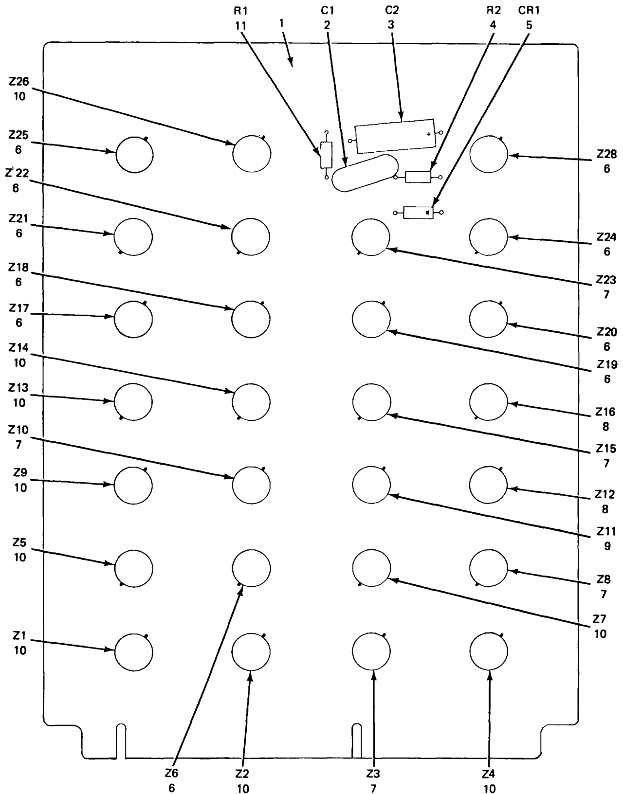
Figure 4. Circuit Card Assembly A1A13.
