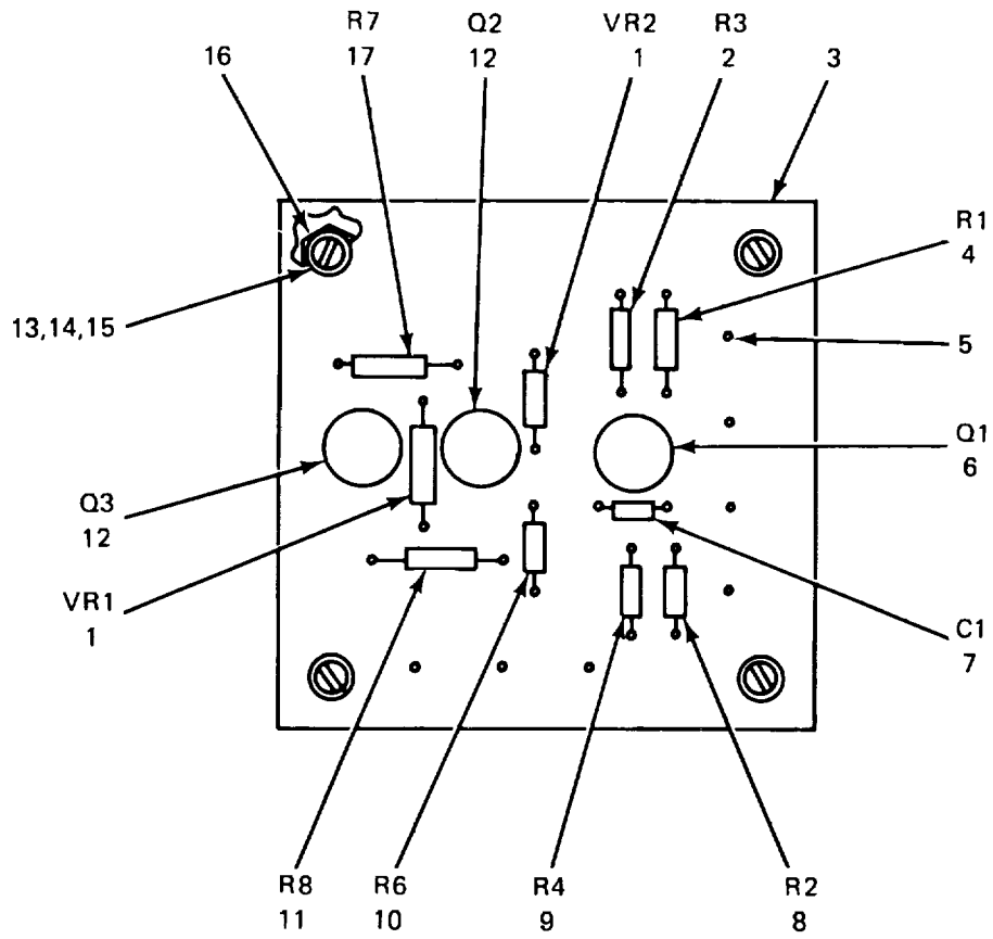
Figure 40. Circuit Card Assembly (890050).
