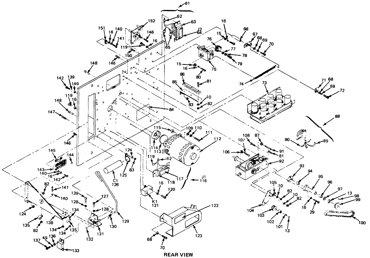
Figure 30. Perforator Assembly (Sheet 2 of 2)
