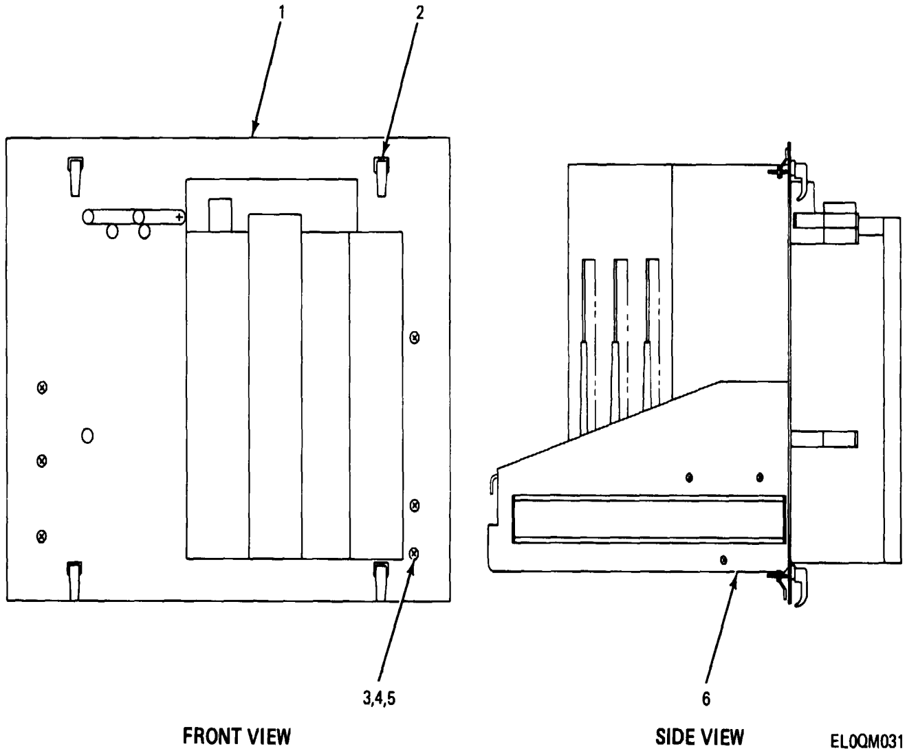
Figure 25. Punch Assembly A4.
