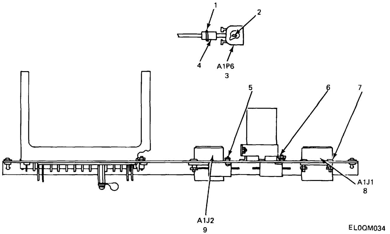
Figure 28. Wiring Harness (A65407-001).
