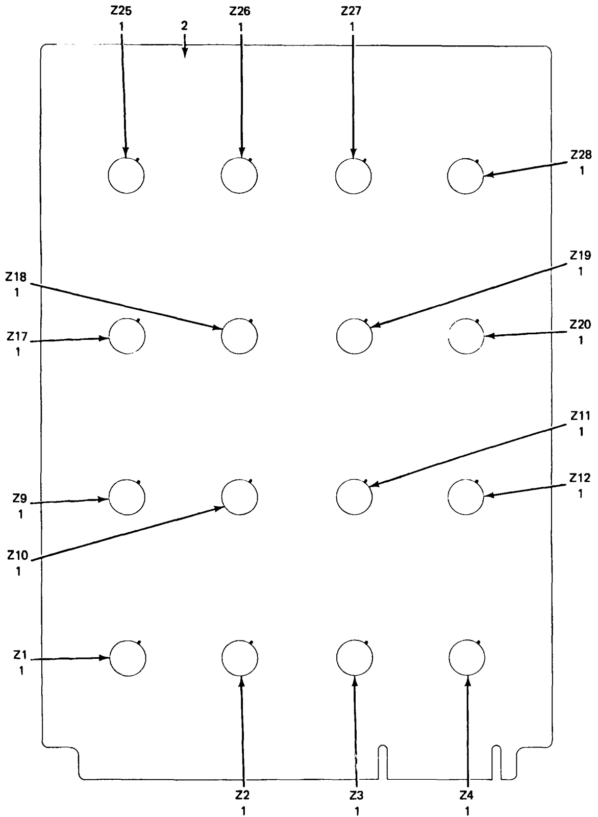
Figure 7. Circuit Card Assembly A1A15.
