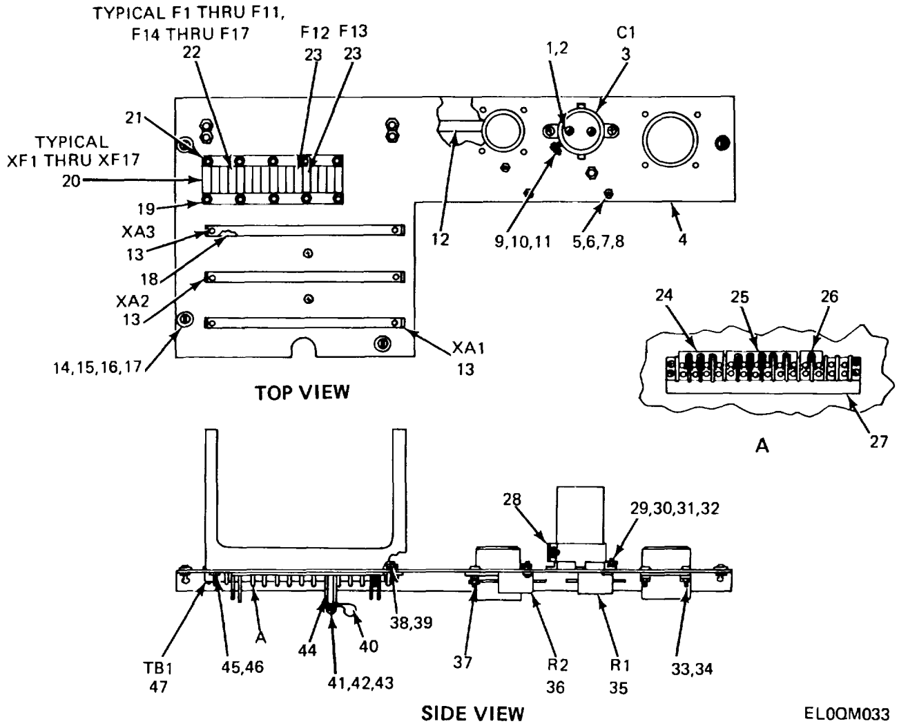
Figure 27. Shelf Assembly.
