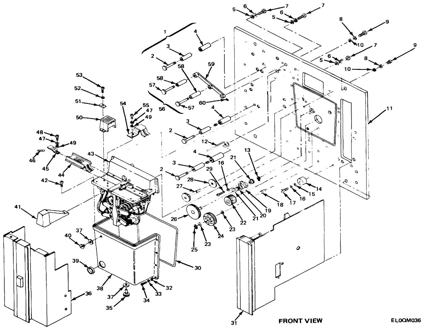
Figure 30. Perforator Assembly (Sheet 1 of 2).
