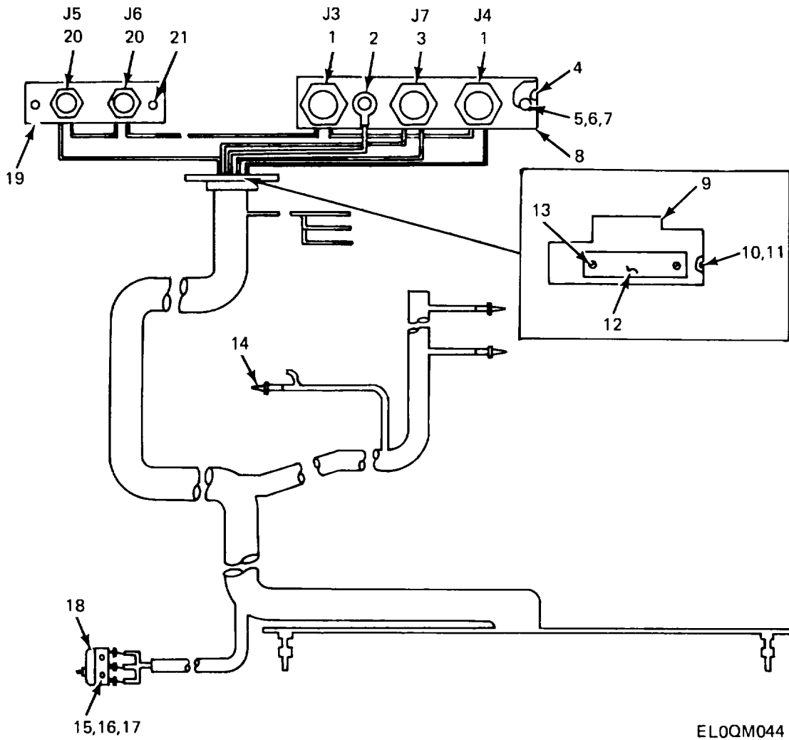
Figure 37. Cable Assembly, Mechanism.
