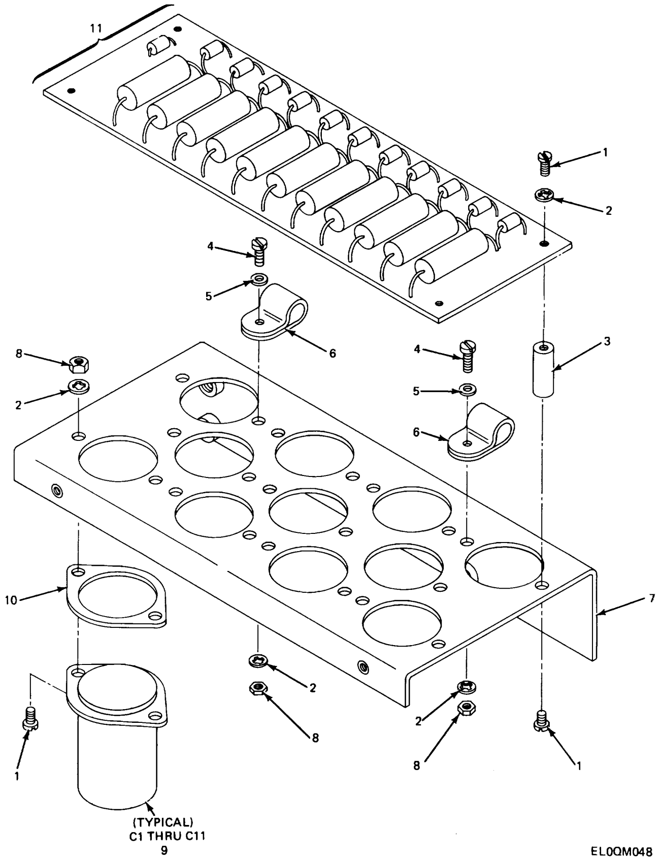
Figure 41. Network Resistance-Capacitance Assembly.
