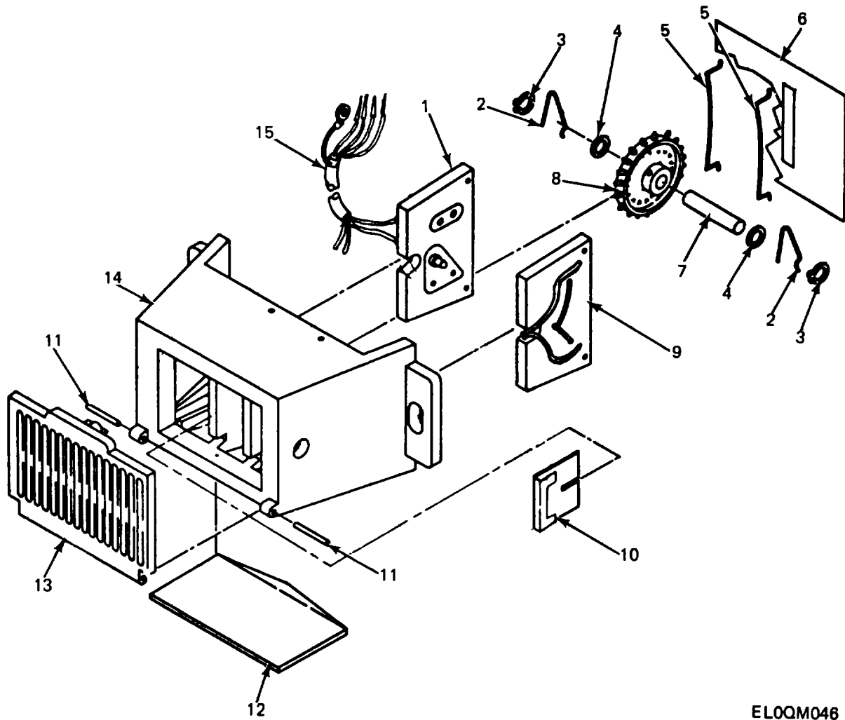
Figure 39. Sensor Assembly, Tape Motion.
