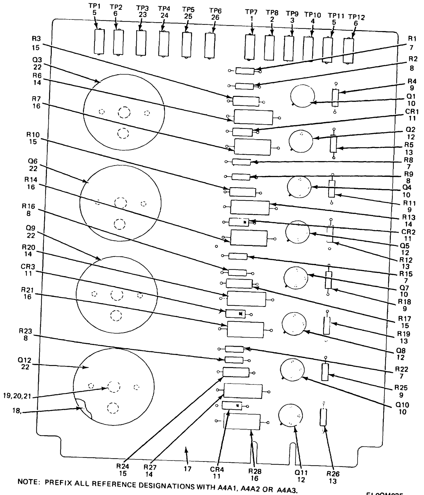
Figure 29. Circuit Card Assembly A4A1.
