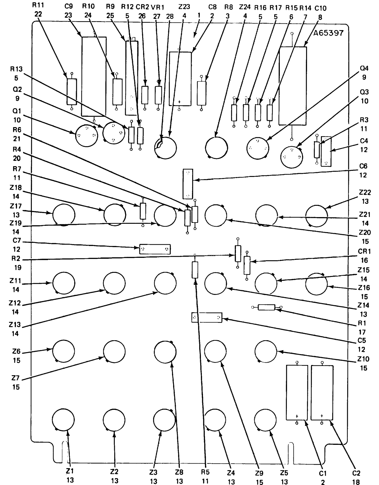
Figure 17. Circuit Card Assembly A1A3.
