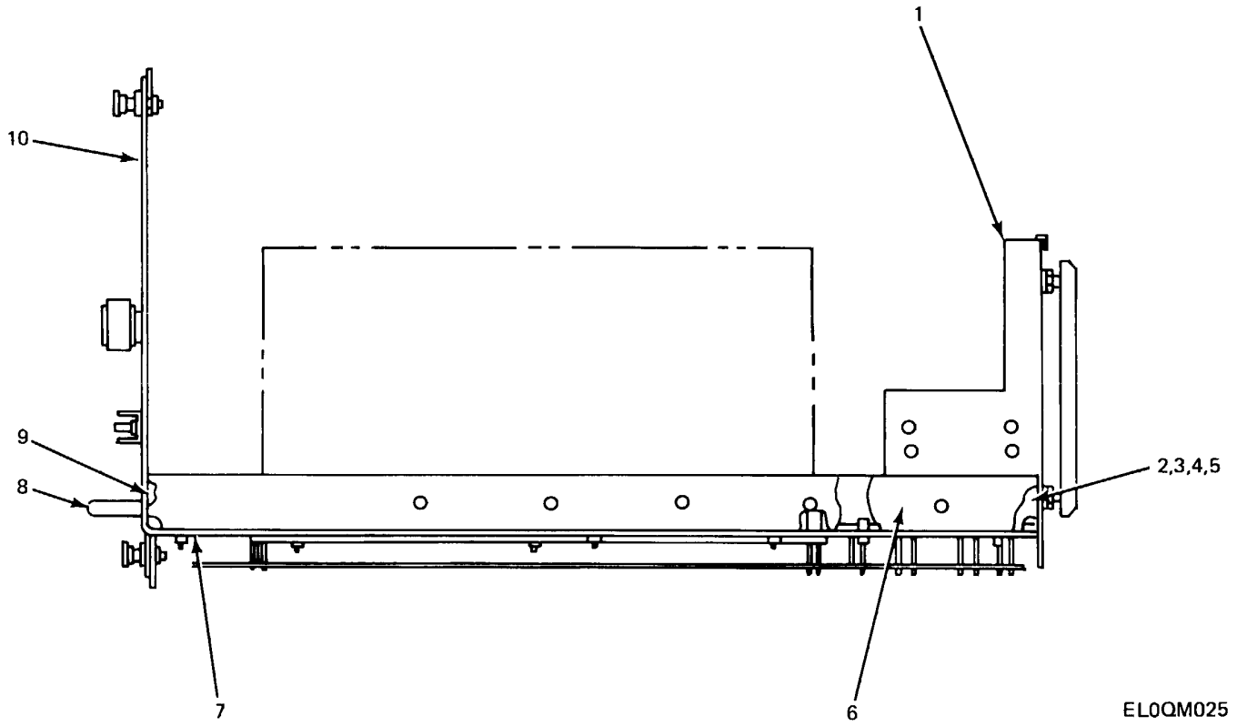
Figure 19. Logic Chassis.
