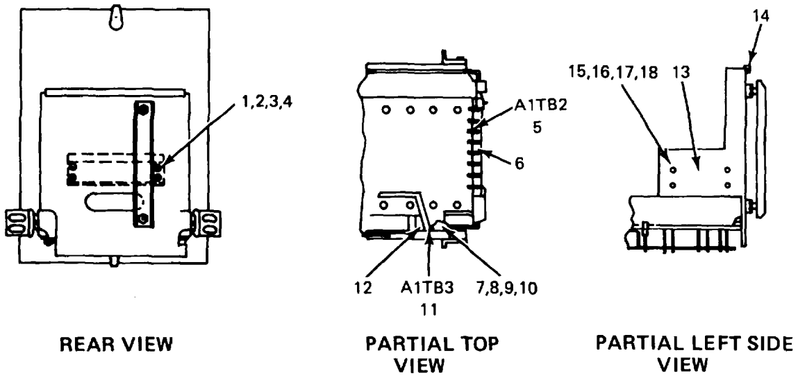
Figure 21. Logic Assembly (A64504-004).
