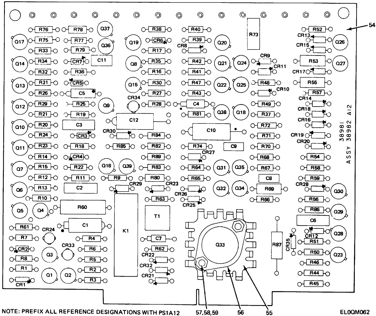
Figure 55. Circuit Card Assembly PS1A12 (Sheet 1 of 3).
