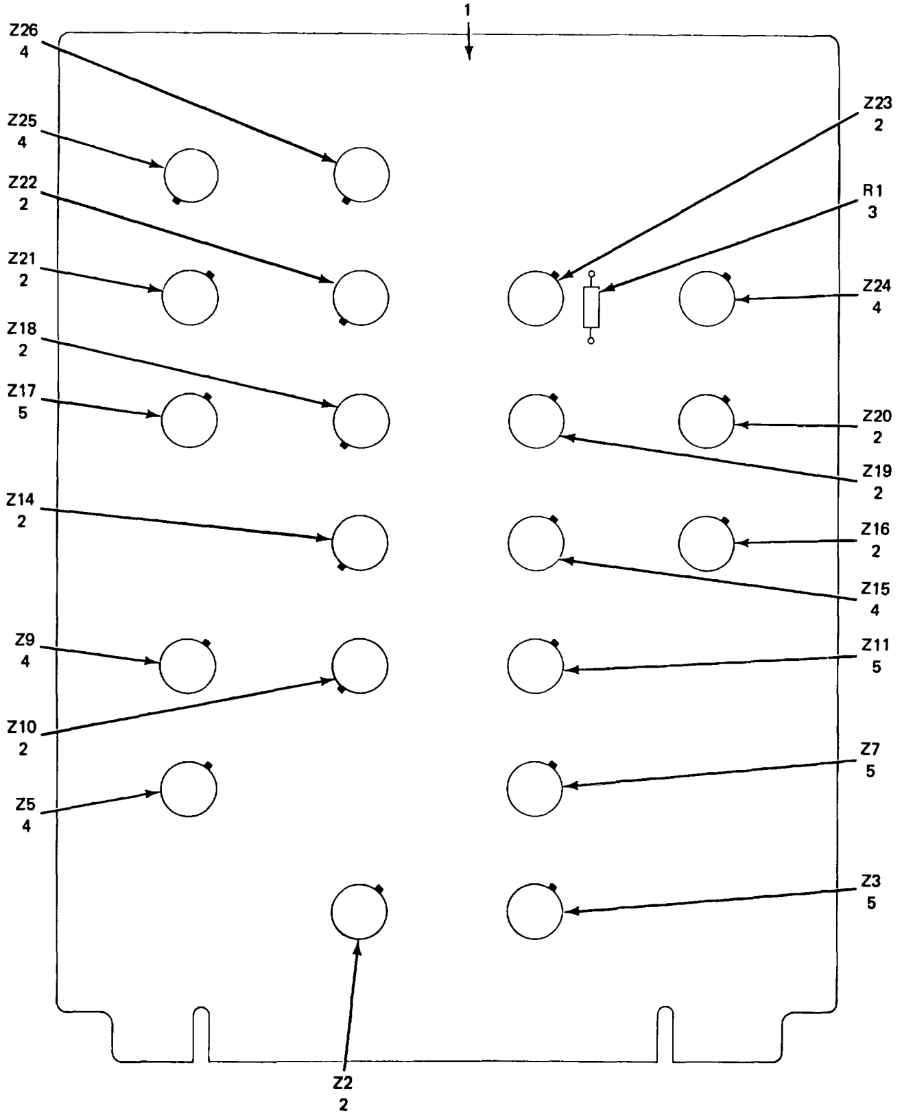
Figure 5. Circuit Card Assembly A1A12.
